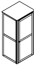
Ref: B - Upper unit Dimension (mm): 710x600x1500 Quantity: 1 pc Box Number: 2
