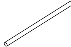
Ref: C - Hanger rod Dimension (mm): Ø29x600 Quantity: 1 pc Box Number: 2
